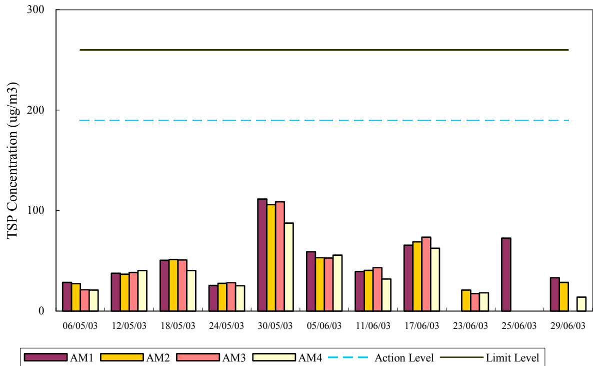
24-hr TSP Air Monitoring Data (May 2003 - June 2003)
