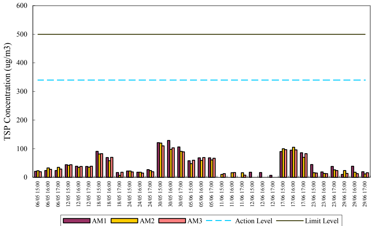
1-hr TSP Air Monitoring Data (May 2003 - June 2003)
