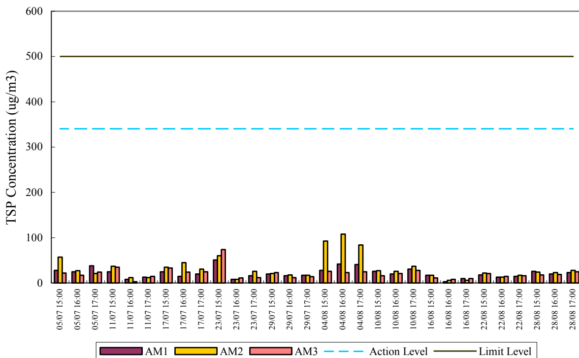
1-hr TSP Air Monitoring Data (July 2003 - August 2003)
