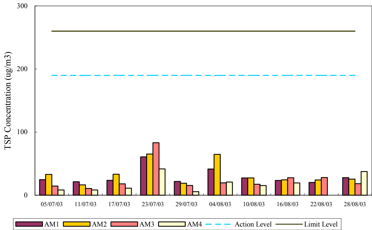
24-hr TSP Air Monitoring Data (July 2003 - August 2003)
