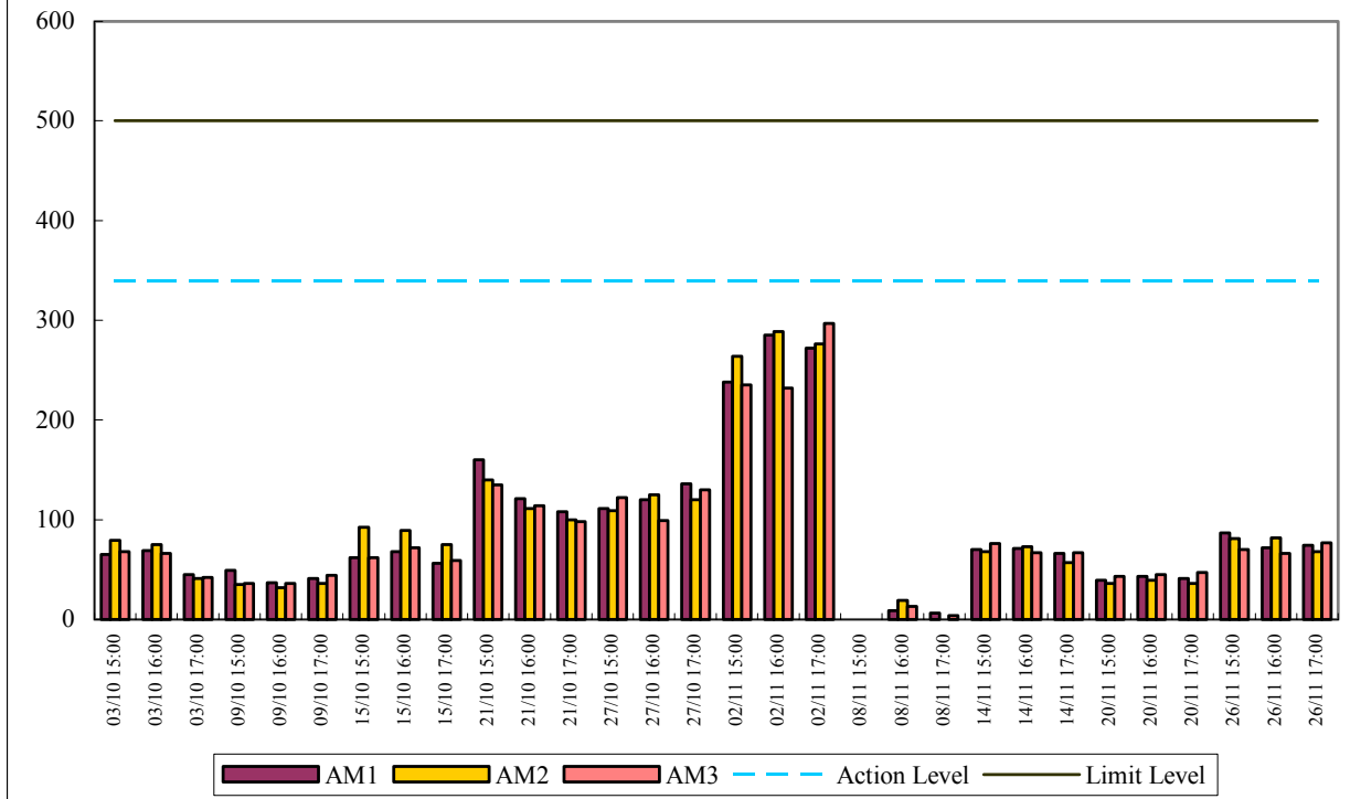
1-hr TSP Air Monitoring Data (October 2003 - November 2003)
