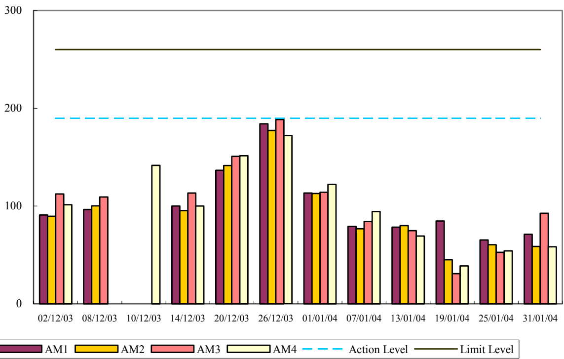
24-hr TSP Air Monitoring Data (December 2003 - January 2004)
