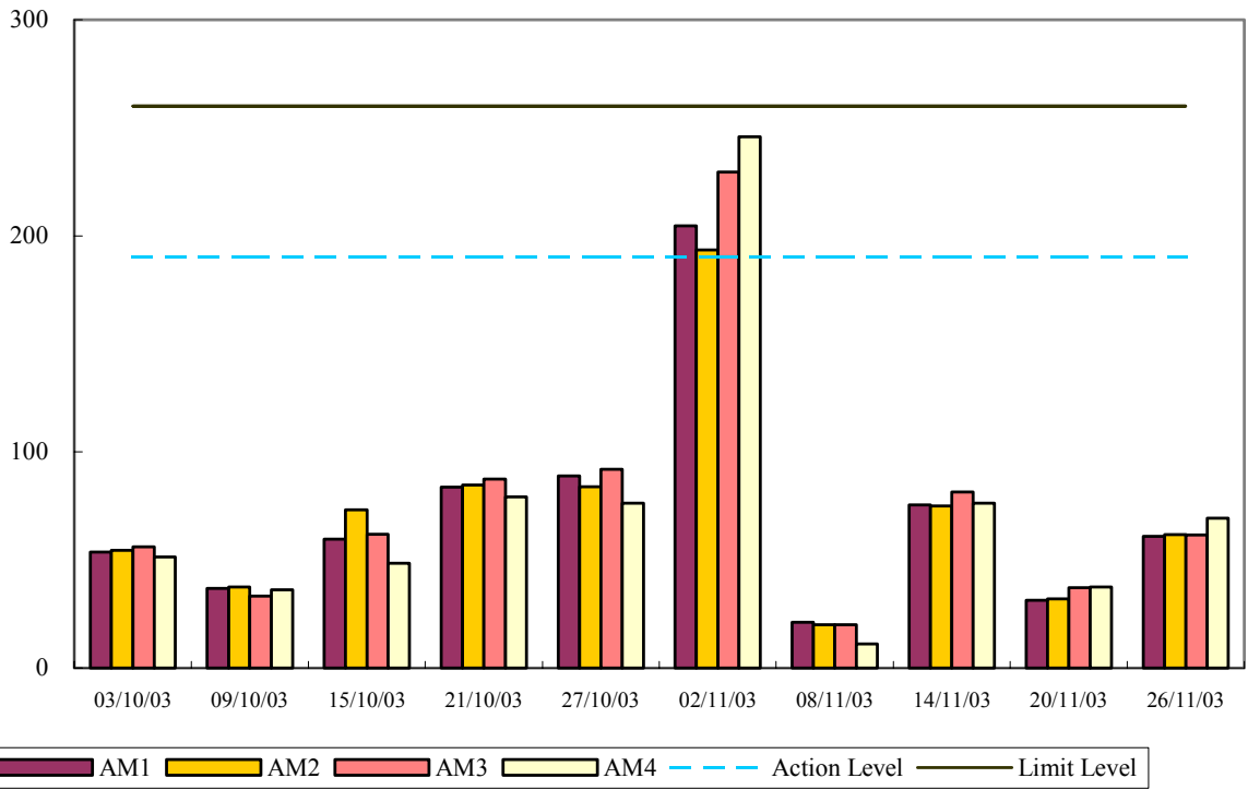
24-hr TSP Air Monitoring Data (October 2003 - November 2003)
