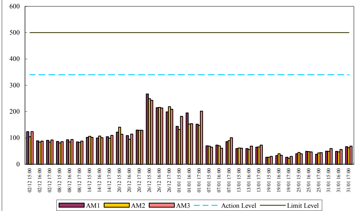
1-hr TSP Air Monitoring Data (December 2003 - January 2004)
