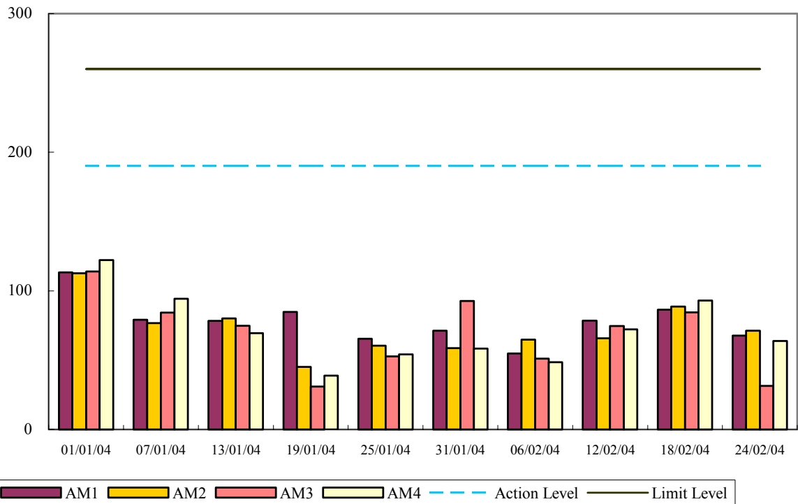
24-hr TSP Air Monitoring Data (January 2004 - February 2004)
