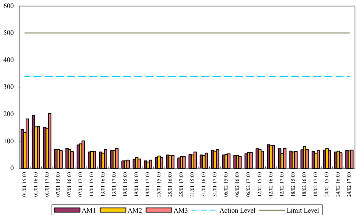
1-hr TSP Air Monitoring Data (January 2004 - February 2004)
