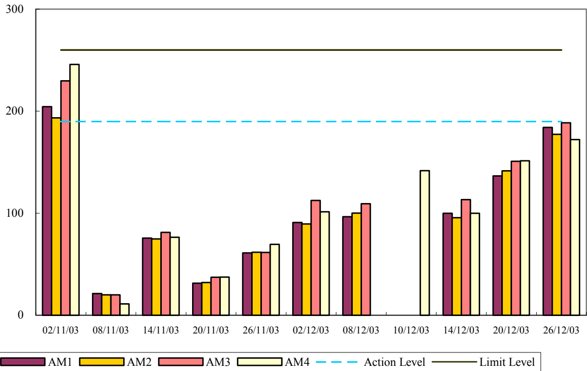
24-hr TSP Air Monitoring Data (November 2003 - December 2003)
