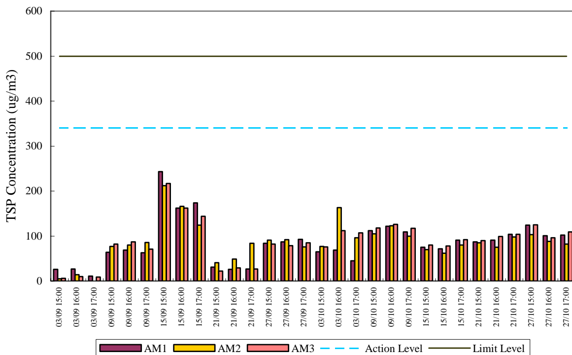
1-hr TSP Air Monitoring Data (September 2004 - October 2004)
