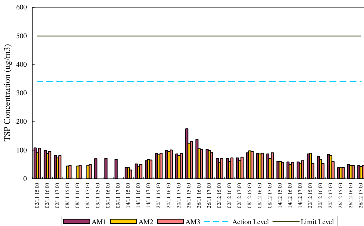
1-hr TSP Air Monitoring Data (November 2004 - December 2004)
