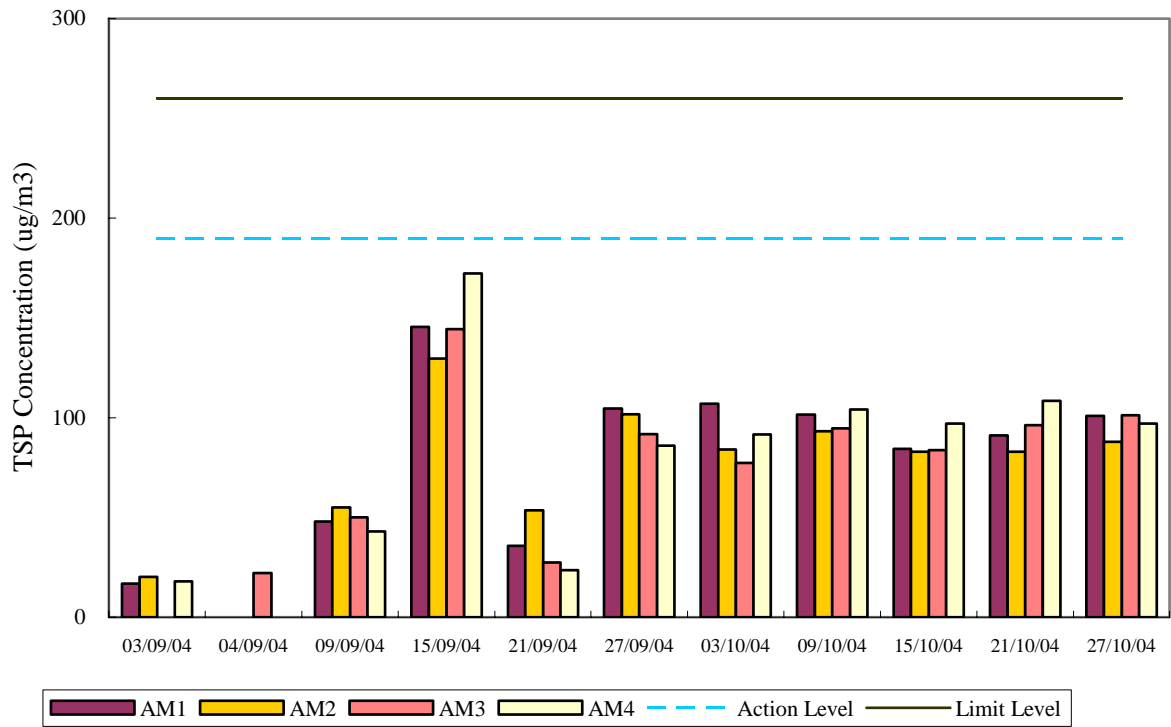
24-hr TSP Air Monitoring Data (September 2004 - October 2004)
