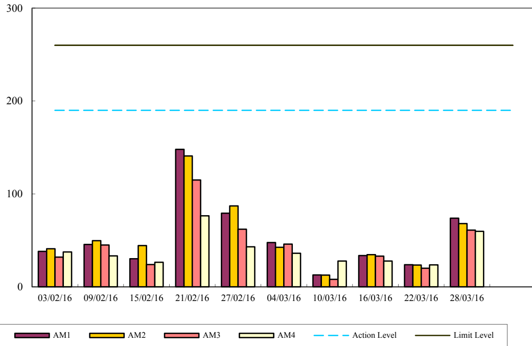
24-hr TSP Air Monitoring Data (February 2016 - March 2016)
