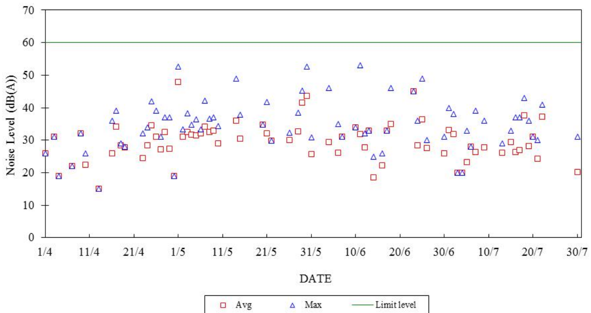
Construction Noise Monitoring in April - July 2017 NSR at School within Tai Wan San Tsuen 07:00-23:00 hrs on Holidays and 19:00-23:00 hrs on All Other Days
