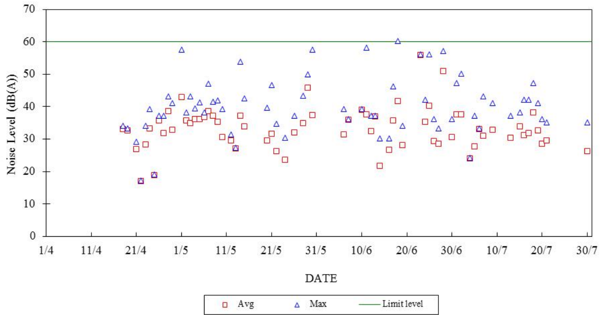
Construction Noise Monitoring in April - July 2017 NSR at Long Tsai Tsuen/Hung Shing Ye 07:00-23:00 hrs on Holidays and 19:00-23:00 hrs on All Other Days
