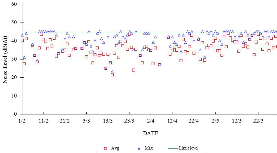
Construction Noise Monitoring in February - May 2019 NSR at Long Tsai Tsuen/Hung Shing Ye 23:00-07:00 hrs of Next Day
