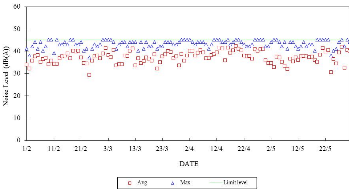
Construction Noise Monitoring in February - May 2019 NSR at School within Tai Wan San Tsuen 23:00-07:00 hrs of Next Day
