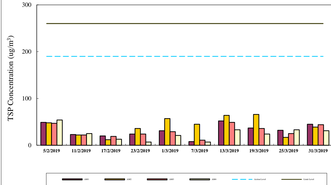
24-hr TSP Air Monitoring Data (February 2019 - March 2019)
