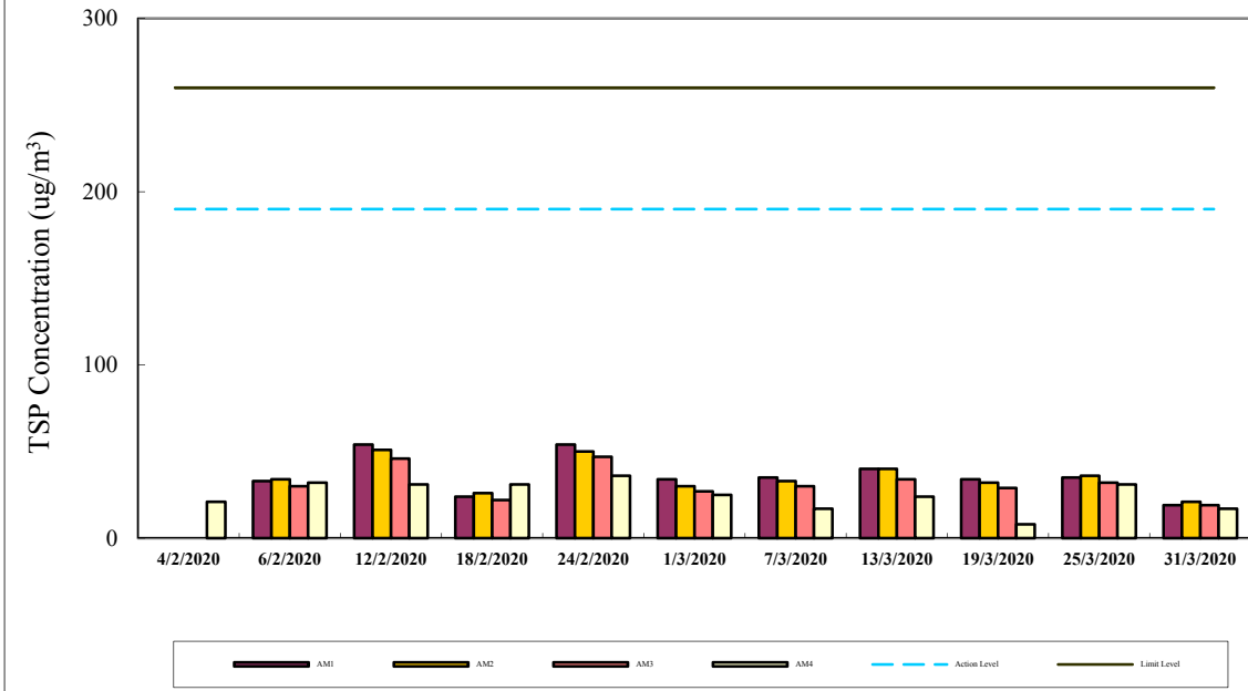
24-hr TSP Air Monitoring Data (February 2020 - March 2020)
