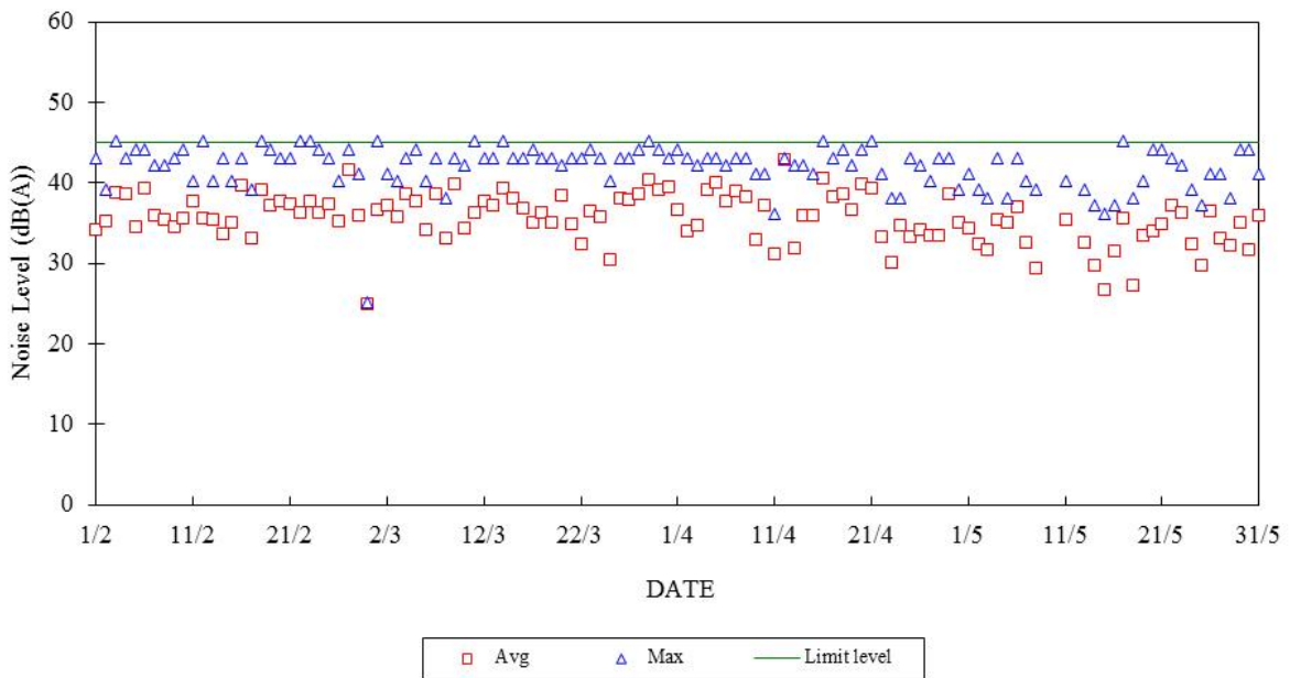
Construction Noise Monitoring in February - May 2020 NSR at School within Tai Wan San Tsuen 23:00-07:00 hrs of Next Day
