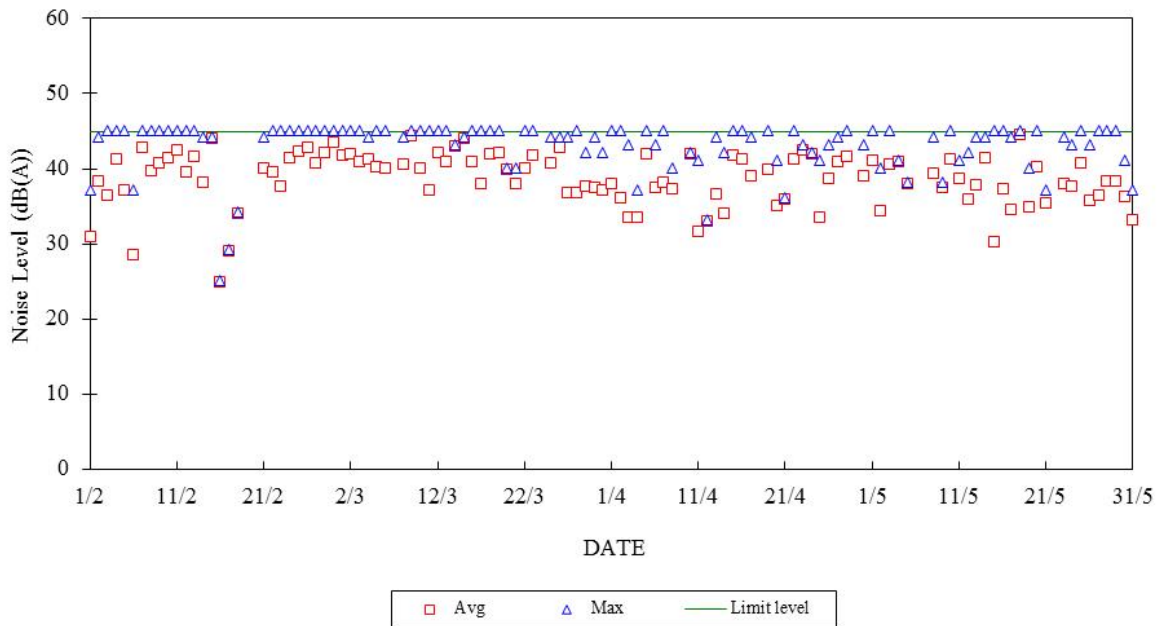
Construction Noise Monitoring in February - May 2020 NSR at Long Tsai Tsuen/Hung Shing Ye 23:00-07:00 hrs of Next Day
