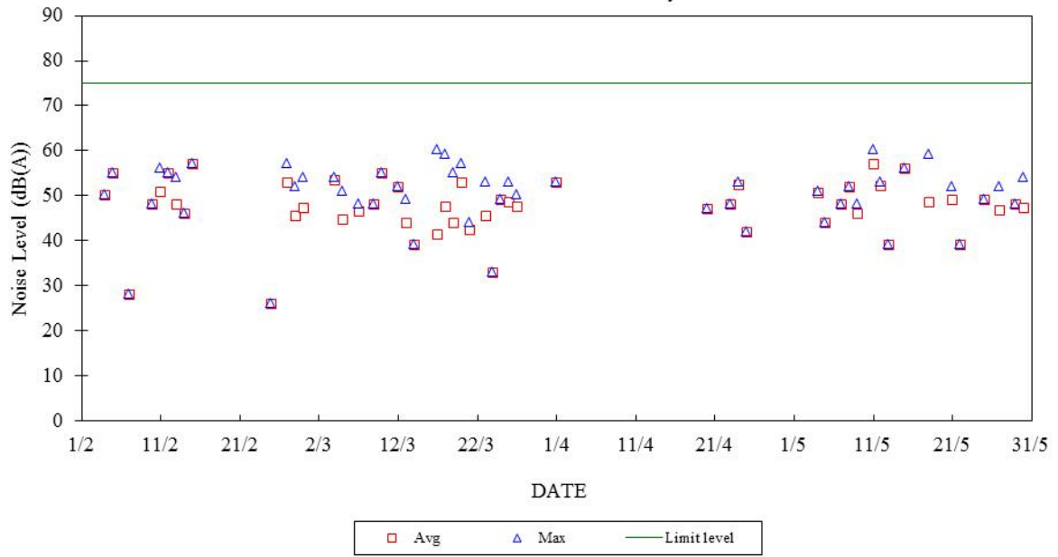
Construction Noise Monitoring in February - May 2020 NSR at Long Tsai Tsuen/Hung Shing Ye 07:00-19:00 hrs on Normal Weekdays
