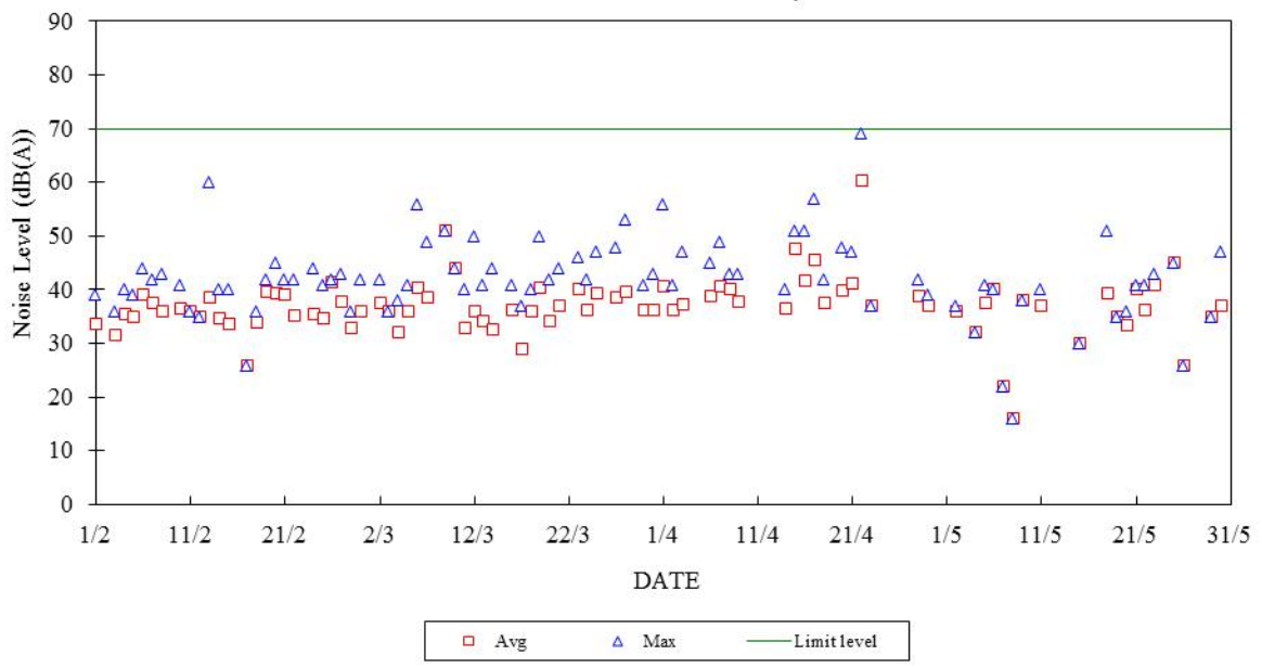
Construction Noise Monitoring in February - May 2020 NSR at School within Tai Wan San Tsuen 07:00-19:00 hrs on Normal Weekdays
