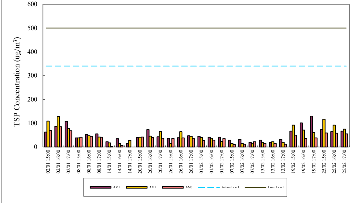
1-hr TSP Air Monitoring Data (January 2023 - February 2023)
