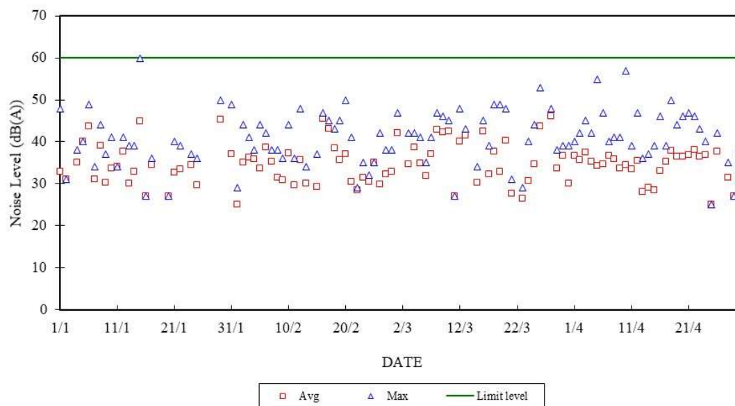
Construction Noise Monitoring in January - April 2023 NSR at School within Tai Wan San Tsuen 07:00-23:00 hrs on Holidays and 19:00-23:00 hrs on All Other Days
