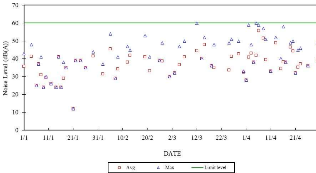
Construction Noise Monitoring in January - April 2023 NSR at Long Tsai Tsuen/Hung Shing Ye 07:00-23:00 hrs on Holidays and 19:00-23:00 hrs on All Other Days
