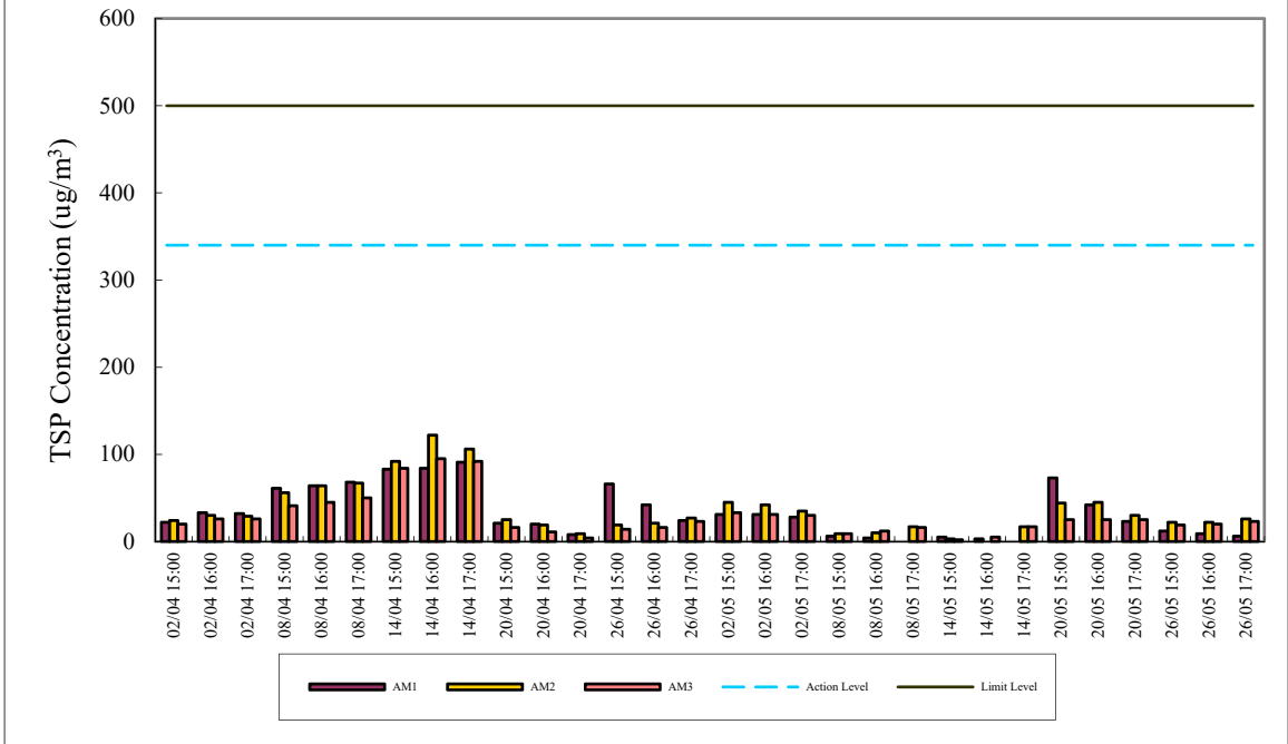
1-hr TSP Air Monitoring Data (April 2023 - May 2023)
