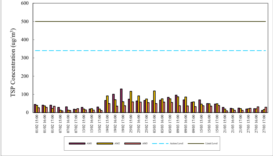
1-hr TSP Air Monitoring Data (February 2023 - March 2023)
