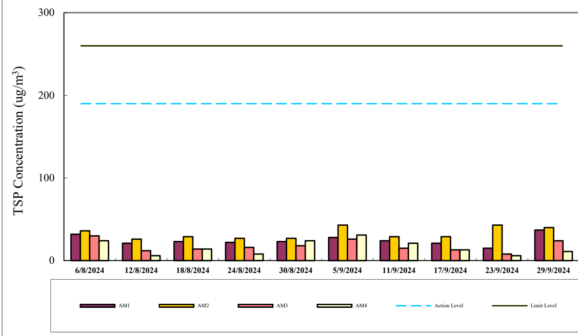
24-hr TSP Air Monitoring Data (August 2024 - September 2024)
