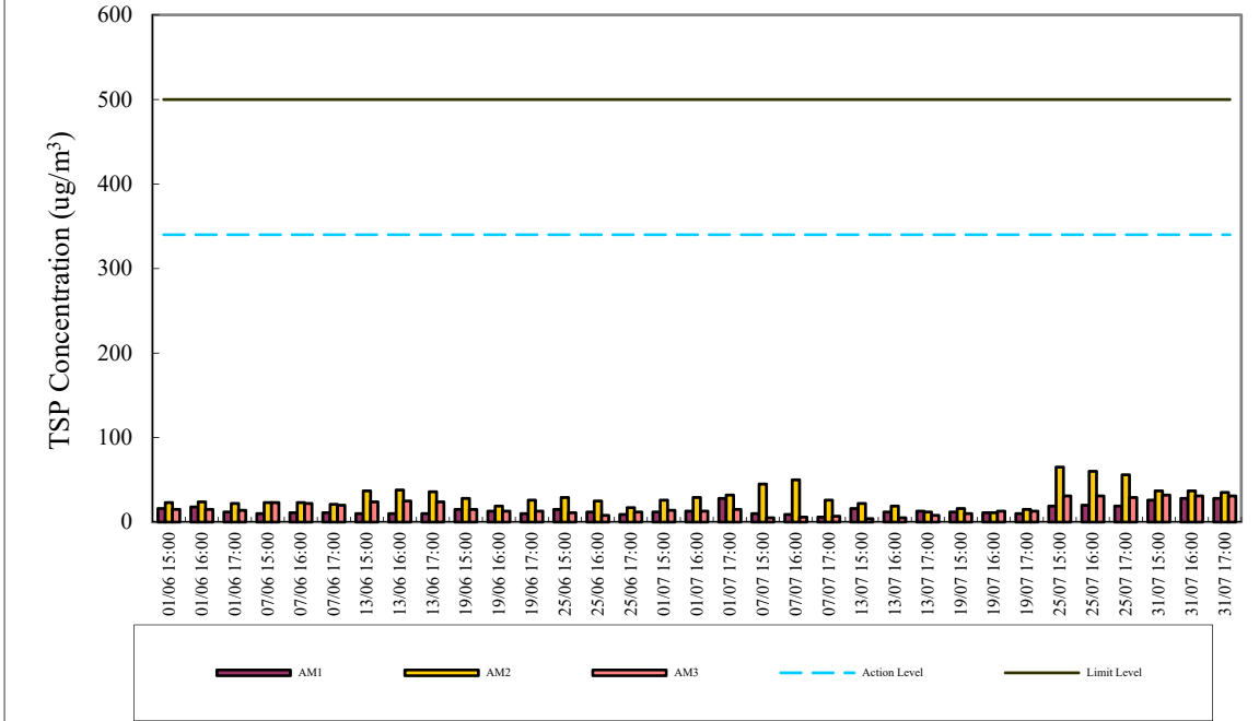
1-hr TSP Air Monitoring Data (June 2024 - July 2024)
