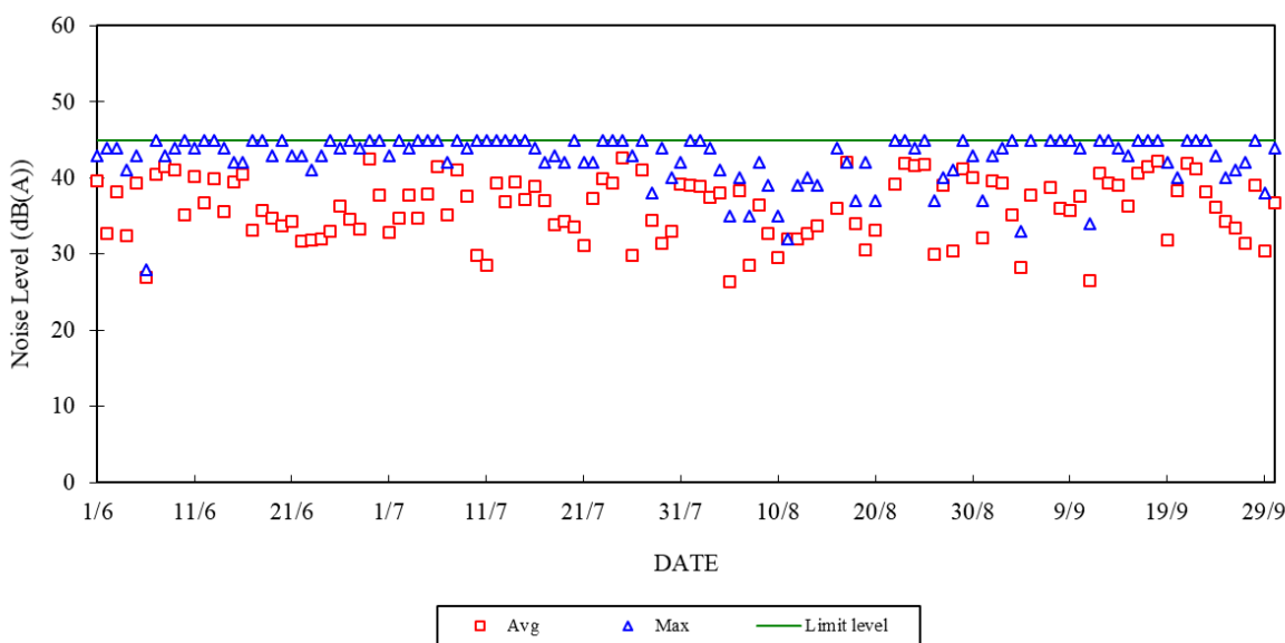
Construction Noise Monitoring in June 2024 - September 2024 NSR at School within Tai Wan San Tsuen 23:00-07:00 hrs of Next Day
