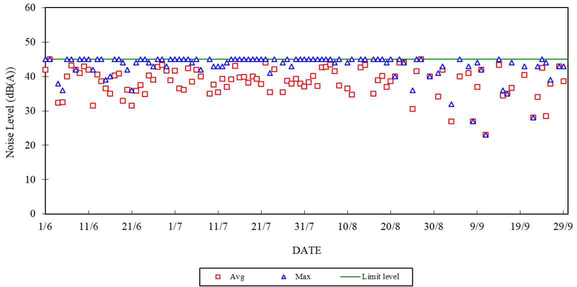
Construction Noise Monitoring in June 2024 - September 2024 NSR at Long Tsai Tsuen/Hung Shing Ye 23:00-07:00 hrs of Next Day
