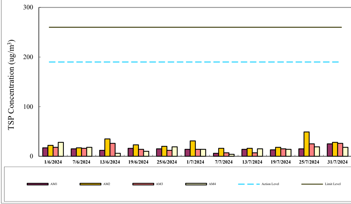
24-hr TSP Air Monitoring Data (June 2024 - July 2024)
