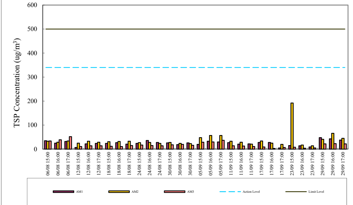
1-hr TSP Air Monitoring Data (August 2024 - September 2024)
