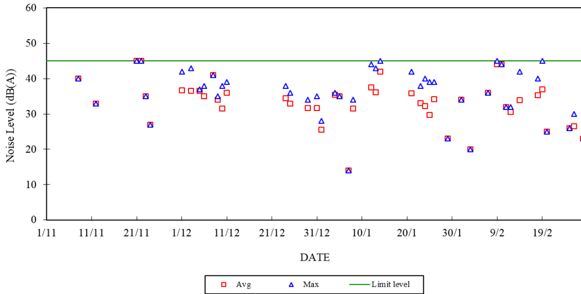
Construction Noise Monitoring in November 2024 - February 2025 NSR at Long Tsai Tsuen/Hung Shing Ye 23:00-07:00 hrs of Next Day
