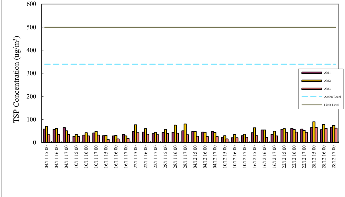
1-hr TSP Air Monitoring Data (November 2024 - December 2024)
