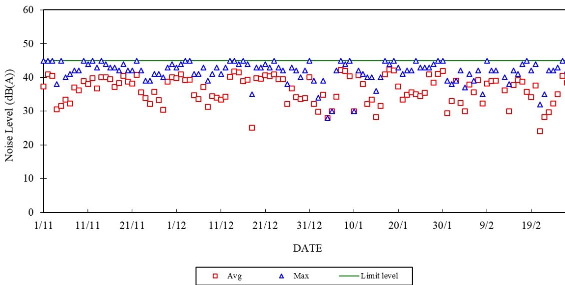
Construction Noise Monitoring in November 2024 - February 2025 NSR at School within Tai Wan San Tsuen 23:00-07:00 hrs of Next Day
