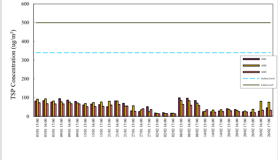
1-hr TSP Air Monitoring Data (January 2025 - February 2025)
