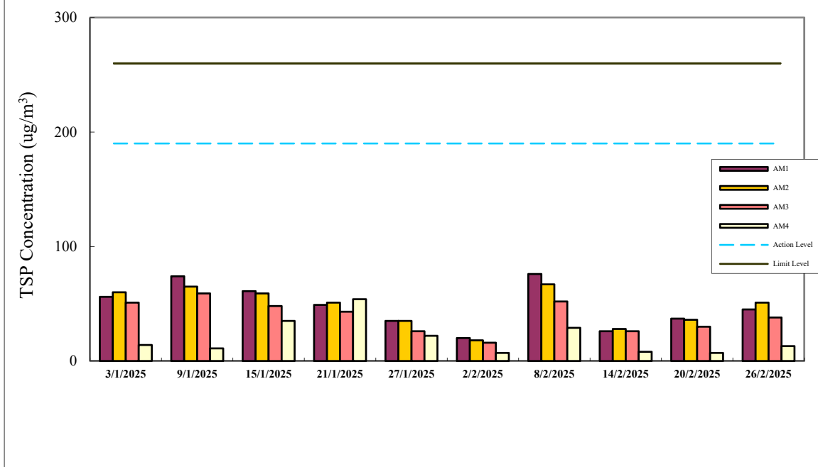
24-hr TSP Air Monitoring Data (January 2025 - February 2025)
