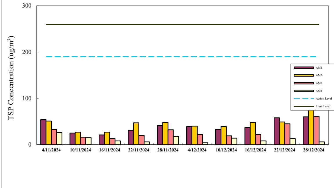
24-hr TSP Air Monitoring Data (November 2024 - December 2024)
