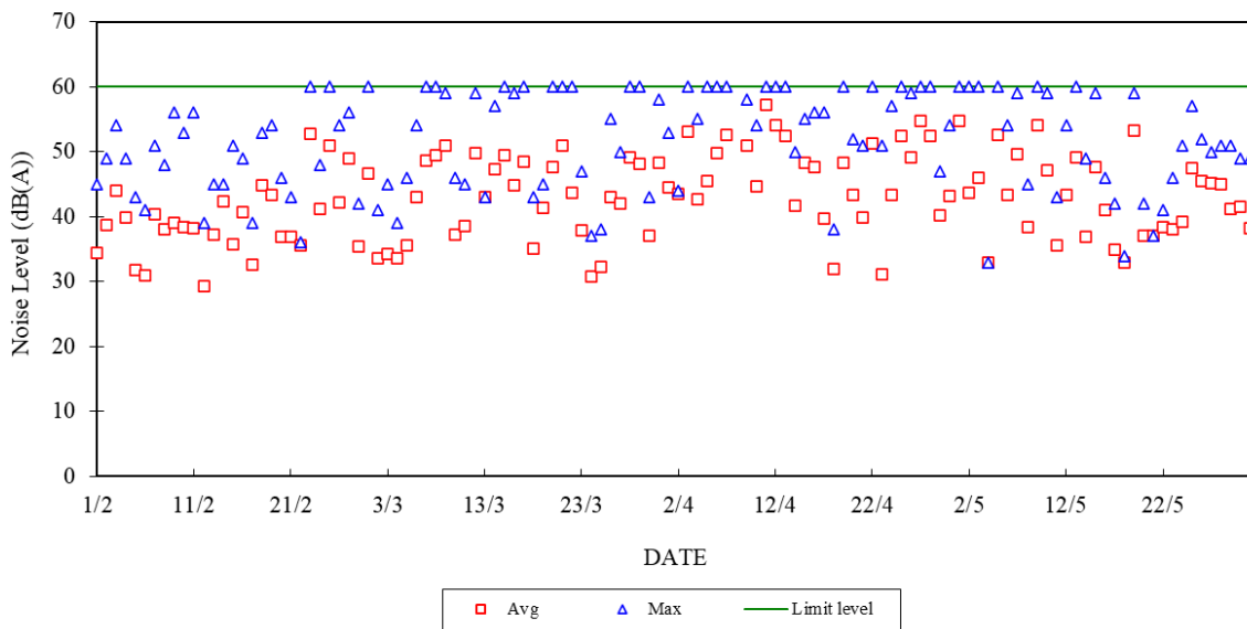
Construction Noise Monitoring in February 2026 - May 2026 NSR at School within Tai Wan San Tsuen 07:00-23:00 hrs on Holidays and 19:00-23:00 hrs on All Other Days
