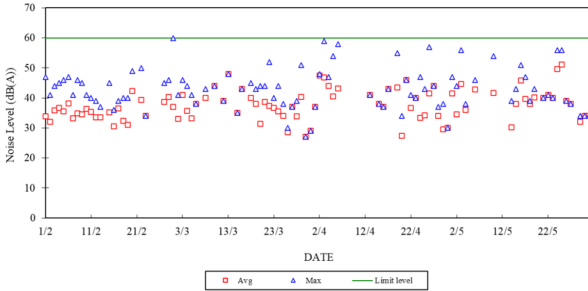
Construction Noise Monitoring in February 2026 - May 2026 NSR at Long Tsai Tsuen/Hung Shing Ye 07:00-23:00 hrs on Holidays and 19:00-23:00 hrs on All Other Days
