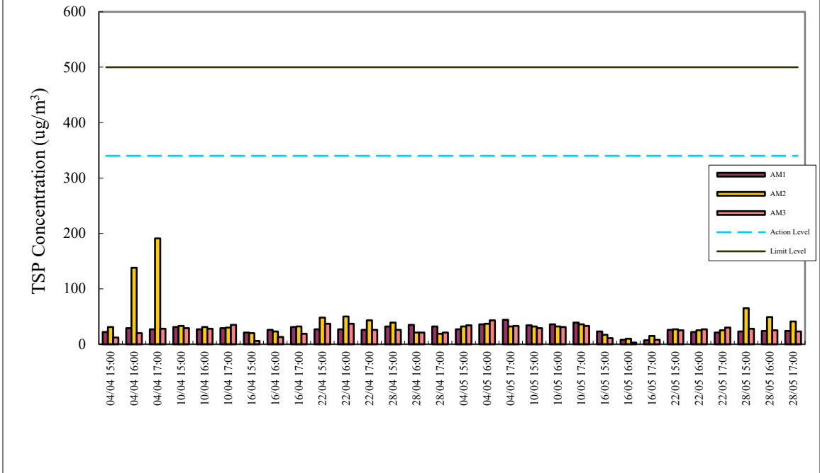
1-hr TSP Air Monitoring Data (April 2026 - May 2026)
