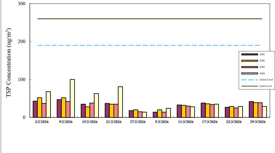
24-hr TSP Air Monitoring Data (April 2026 - May 2026)
